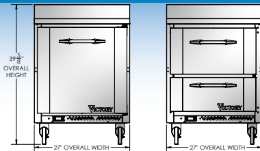
VWR27HC/VWF27HC VWRD27HC-2/VWF- D27HC-2
