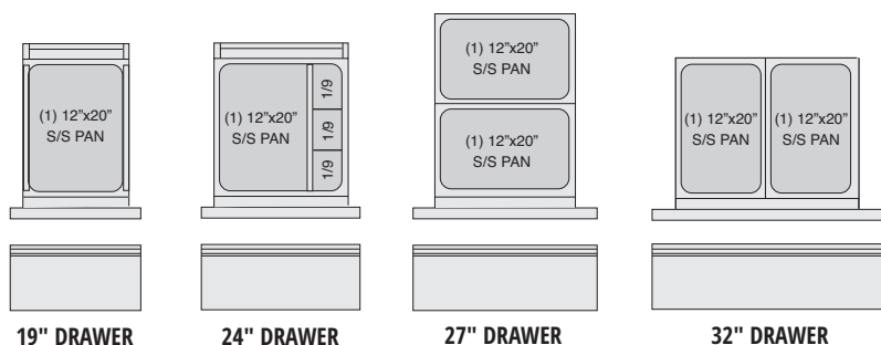
Drawer configurations for BUCMP and BSTMP series.
