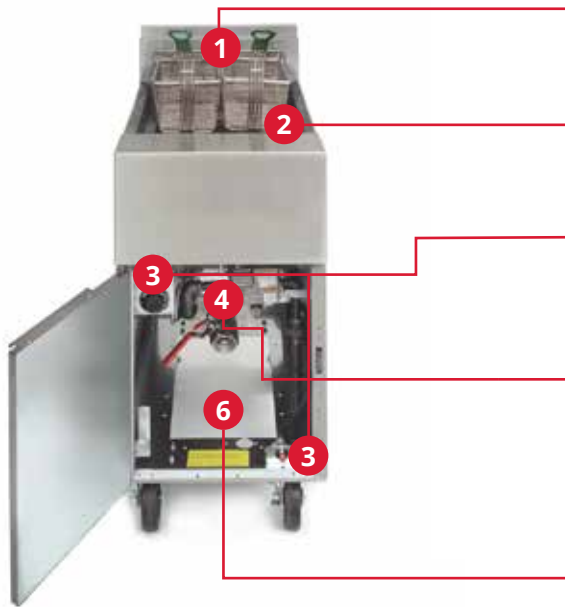
GF14 fryer shown with optional and Piezo ignitor
